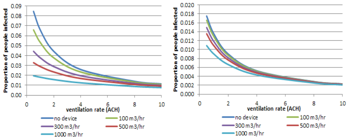
Figure 4: Simulation from Wells-Riley model for airborne transmission over a 2 hour period, 10 quanta/hr and breathing rate of 10 l/min. Results for device flow rates between 100 and 1000 m3/hr in a 100 m3 room (left) and 500 m3 room (right).
